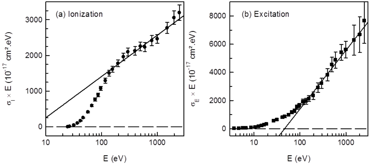
FIG. 9. Bethe-plot of the (a) total ionization cross-section ( \bullet \sigma_I ) and of the (b) total excitation cross-section ( \blacksquare \sigma_E ) of CD_3^+(CH_3^+) . Each full line results from a linear fit using the Bethe-Born formula.
