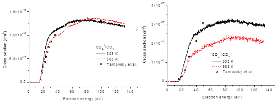
FIG. 4. Partial ionization cross-sections for electron impact ionization of CD_3^+/CD_4 and CD_2^+/CD_4 measured at the gas temperature of 303 K and 683 K.
