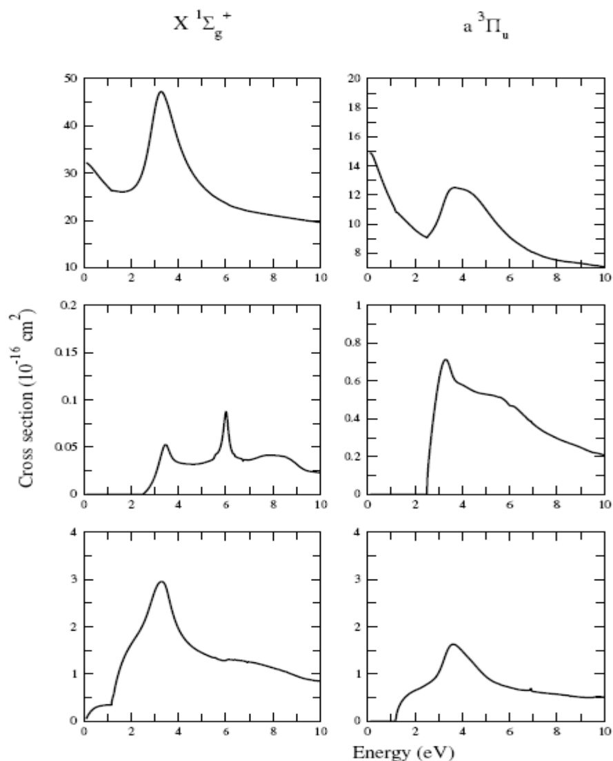
FIG. 1. Electron impact cross-sections for the C_2 molecule at its equilibrium geometry as calculated by Halmova et al [18]. The left hand panels are for molecules starting in the X^1\Sigma_g^+ ground state and the right hand panels are for molecules starting in the low-lying a^3\Pi_u metastable state. The top row is the total cross-section as a function of energy. The second row is for excitation to the d^3\Pi_u state and the lower panels are for excitation to all other states.
