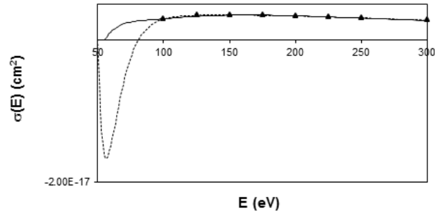
FIG. 1. Example of negative slope of cross-section, vs. electron energy, at threshold in original database, shown for double ionization of C_2H_2 , with E_{th}=I_p=53.4 eV. Triangles: original data, from [14]. dotted line: original fit, loc.cit., solid line: corrected fit according to procedure described in text.
