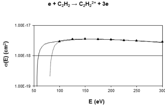
FIG. 2. same as Figure 1, but logarithmic scale for cross-section.
