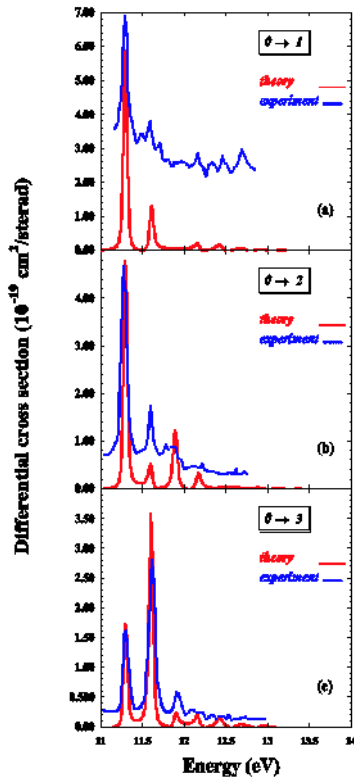
FIG. 6. RVE cross sections for the 0 \rightarrow v_f = 1-3 excitation.
