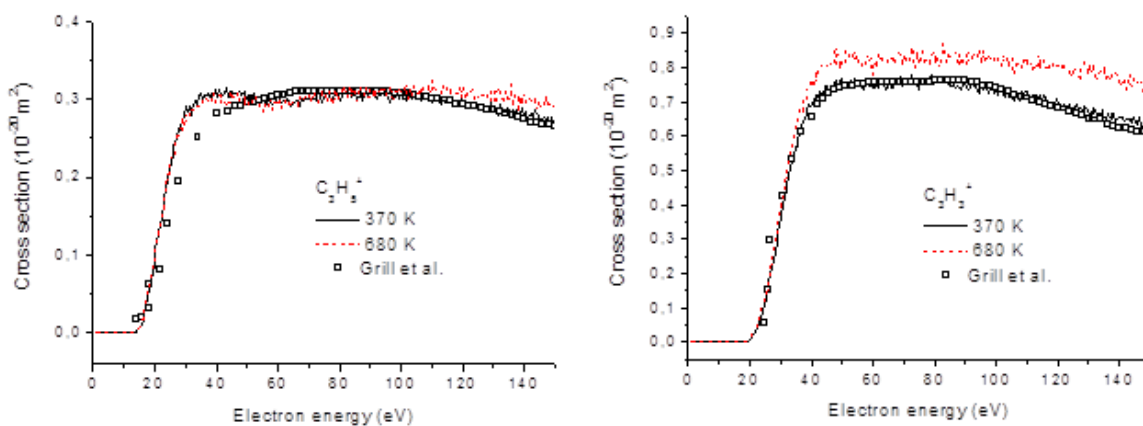
FIG. 21. Absolute partial ionization cross-sections for formation of C_3H_5^+ / C_3H_8 and C_3H_3^+ / C_3H_8 measured at the gas temperatures of 370 K and 680 K.
