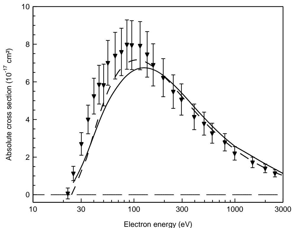
FIG. 5. Total ionization cross-sections ( \sigma_I ) for electron impact upon CD^+ versus electron energy: \blacktriangledown , present measurements; \text{—} , DM formalism [7]; \text{-- --} , BEB model [6].
