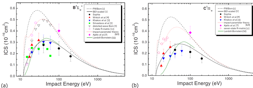
FIG. 8. Integral cross-sections of electronic excitations ( 10^{-16} \text{ cm}^2 ) plotted for the (a) B^1\Sigma^+_u and (b) C^1\Pi_u electronic states. For detailed information, reference should be made to Ref. [39].
