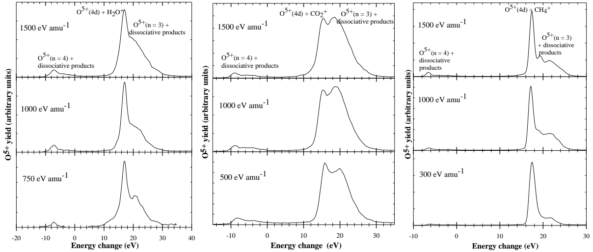
FIG. 22. Energy change spectra for one-electron capture by O 6+ ions in H 2 O, CO 2 and CH 4 (from [7]).
