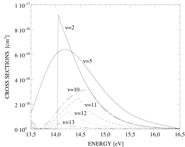
FIG. 6. High energy trends of selected cross-sections for the D_2(\nu) Werner process (see text).
