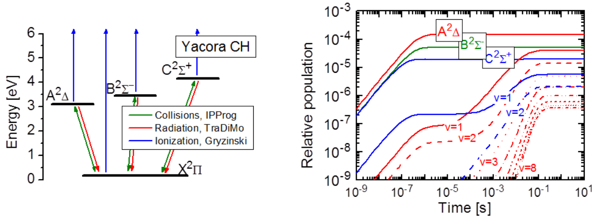
FIG. 9. Left: sketch of the levels used for the CR modelling of CH radiation. Right: equilibrium population density for different excites states of CH ( T_e = 3 eV, n_e = 10^{17} m -3 ).
