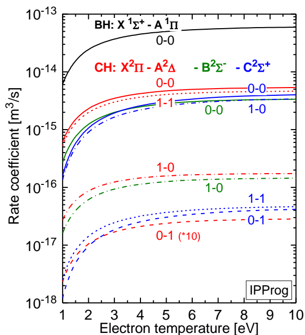
FIG. 8. Vibrationally resolved excitation rate coefficients calculated with IPProg for the ground state of CH into the first electronic states A, B and C as well as for BH the X to A, 0-0 transition.
