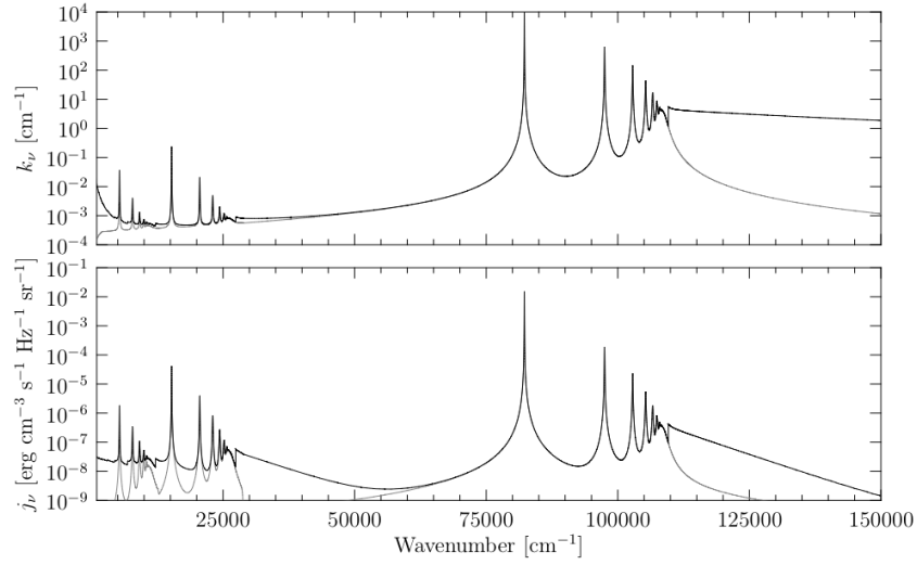
FIG. 11. Absorption, \kappa'_\nu , and emission, j_\nu , coefficients for the (H, H^+, e) . Plasma at thermodynamic equilibrium, T=10\,000 K, p=1 torr. (solid line) total spectrum, (gray-line) bound-bound contribution.
