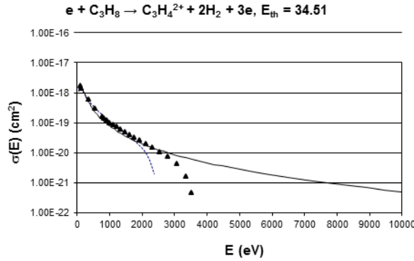
FIG. 3. Example of negative cross-sections at large electron energies in original database, shown here for double ionization of C_3H_8 . Triangles: original data, from [14]. dotted line: original fit, loc.cit., solid line: corrected fit according to procedure described in text.
