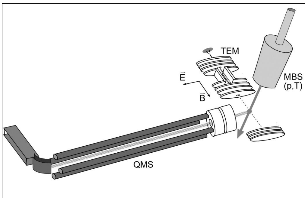
FIG. 1. Schematic view of the experimental setup showing the Effusive Molecular Beam Source (EMBS), Trochoidal Electron Monochromator (TEM) and Quadrupole Mass Spectrometer (QMS).
