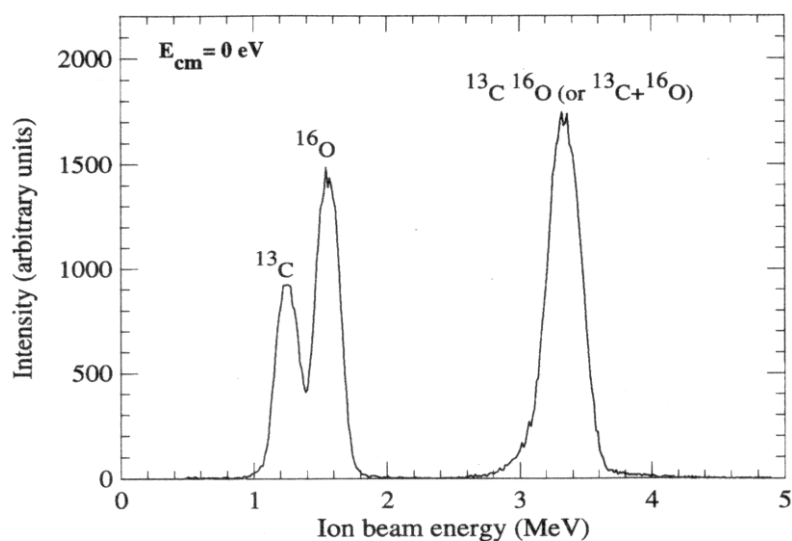
FIG. 2. Pulse height spectrum taken recorded at CRYRING in a study of ^{13}\text{CO}^+ . The C and O peaks derive from collisions of \text{CO}^+ with residual gas molecules, whereas the peak at C + O is totally dominated (>95%) by dissociative recombination events. It occurs at an energy corresponding to the full beam energy of 3.4 MeV (reprinted from Rosén et al. 1998).
