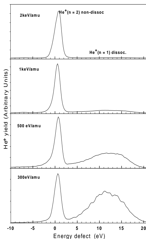
FIG. 16. Energy change spectra for one-electron capture by \text{He}^{2+} ions in \text{CH}_4 (from [5]).
