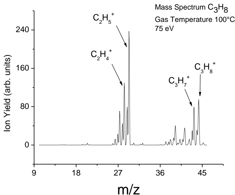
FIG. 19. Mass spectrum of C 3 H 8 measured at the gas temperature of 100°C and the electron energy of 75 eV. The four most abundant peaks are assigned to the corresponding cations.
