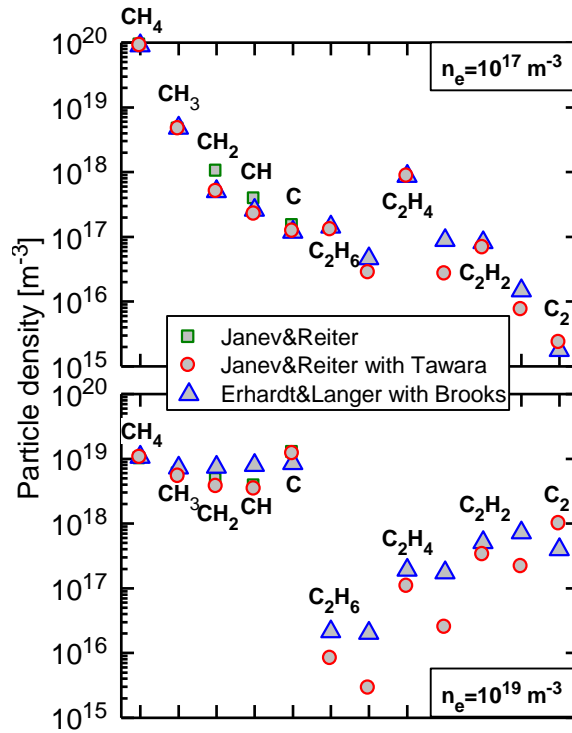
FIG. 12. Comparison of the results from the YACORA dissociation model for methane (using the different input data sets described in the text) at two different electron densities for T_e = 4 eV.
