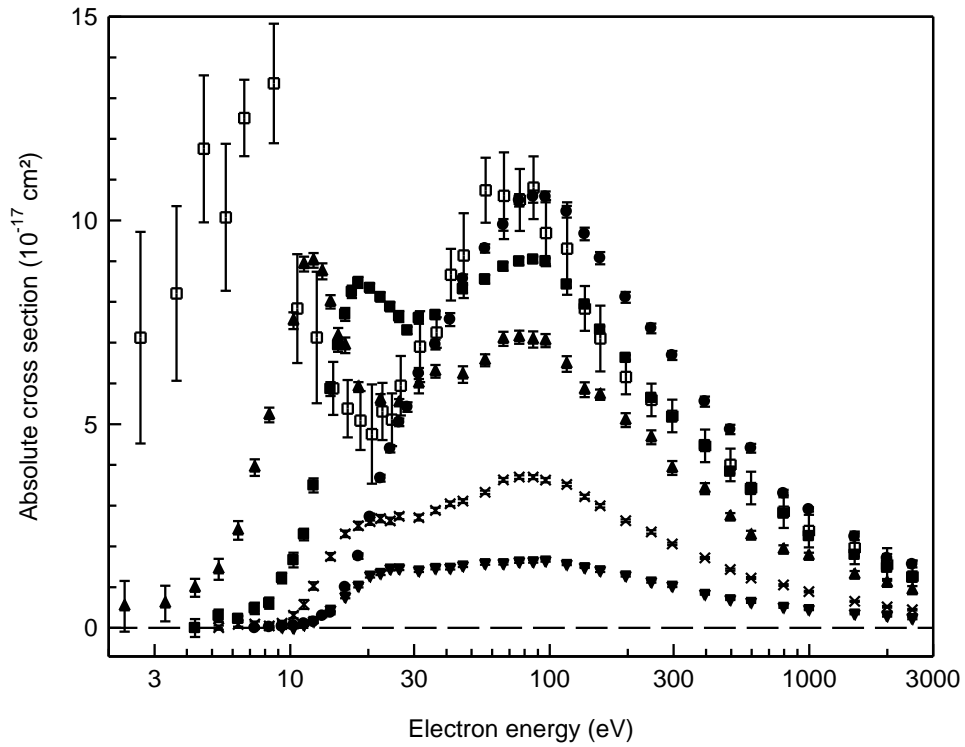
FIG. 4. Absolute total cross-sections for electron impact upon CD_4^+ , versus the electron energy for: D^+ ( \sigma_{41} ; ●), D_2^+ ( \sigma_{42} ; ▼), C^+ ( \sigma_{43} ; ×), CD^+ ( \sigma_{44} ; ■), CD_2^+ ( \sigma_{45} ; ▲) and CD_3^+ ( \sigma_{46} ; □).
