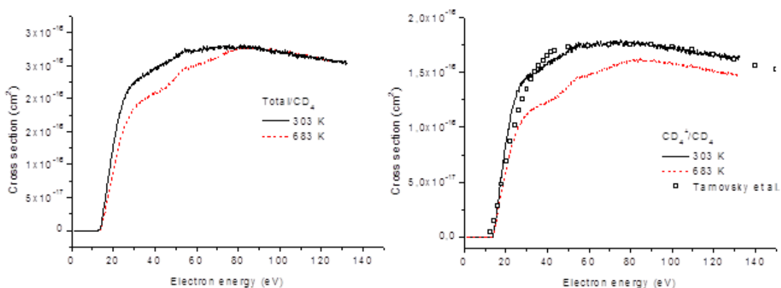
FIG. 3. Total cross-section for electron impact ionization (does not include D + , D 2 + contribution) of CD 4 and partial ionization cross-sections CD 4 + /CD 4 measured at the gas temperature 303 K and 683 K.
