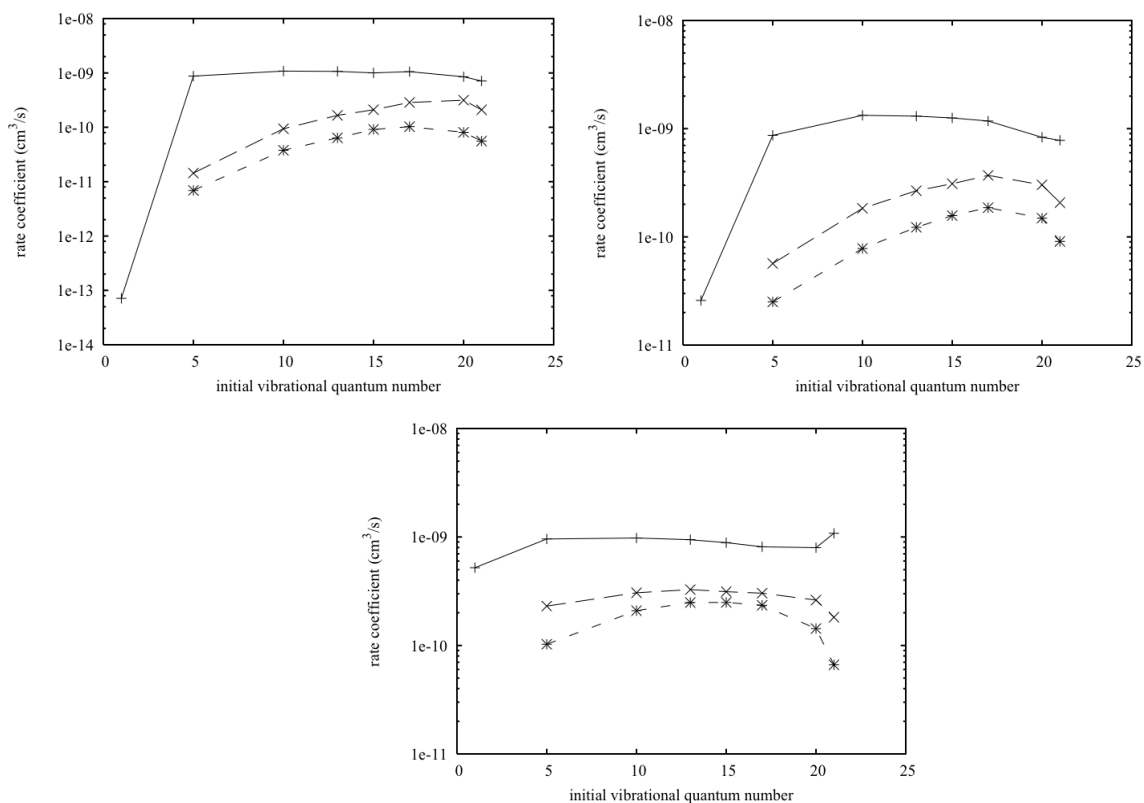
FIG. 3. Deuterium vibrational deactivation rate coefficients as a function of initial vibrational quantum number, at T=300\text{ K} (left higher panel), T=1\,000\text{ K} (right higher panel), T=5\,000\text{ K} (lower panel). (+) v \rightarrow v-1 , (x) v \rightarrow v-2 , (*) v \rightarrow v-5 .
