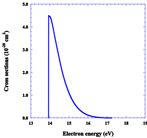
FIG. 9. DEA cross-sections as a function of the incident energy
