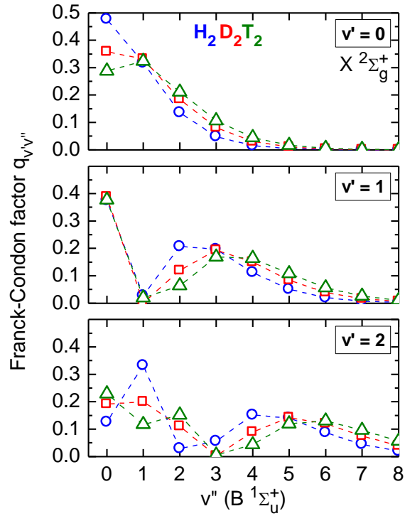
FIG. 1. Franck-Condon factors for the vibrational transitions from the first electronically excited state of H_2 , D_2 and T_2 molecules ( B , v''=0-8 ) to the ground state of the respective molecular ion ( X , v'=0, 1 , and 2).
