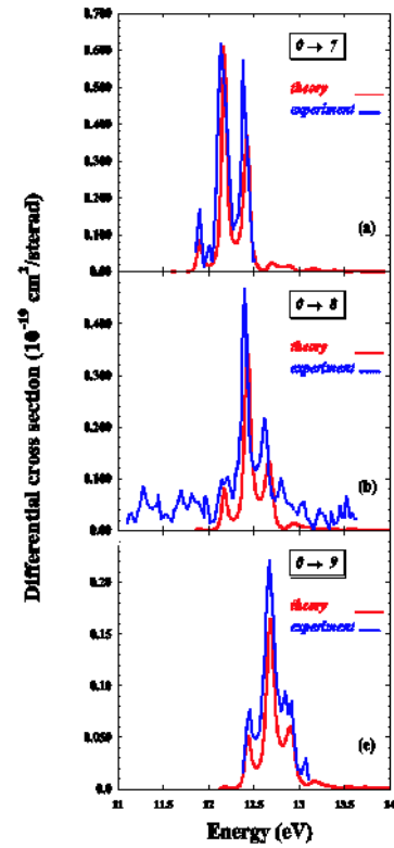
FIG. 8. RVE cross sections for the 0 \rightarrow v_f = 7-9 excitation.
