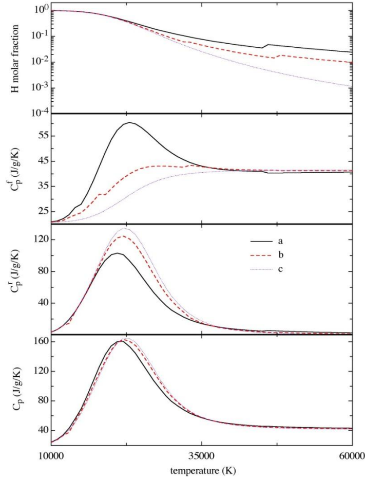
FIG. 8. Molar fraction of hydrogen atom and frozen ( C_p^f ), reactive ( C_p^r ) and total ( C_p ) specific heat of H, H^+ , e mixture as a function of the gas temperature for pressure P=100 atm. (curves a) with Debye-Hückel levels, (curves b) with Coulomb levels, (curves c) only ground state.
