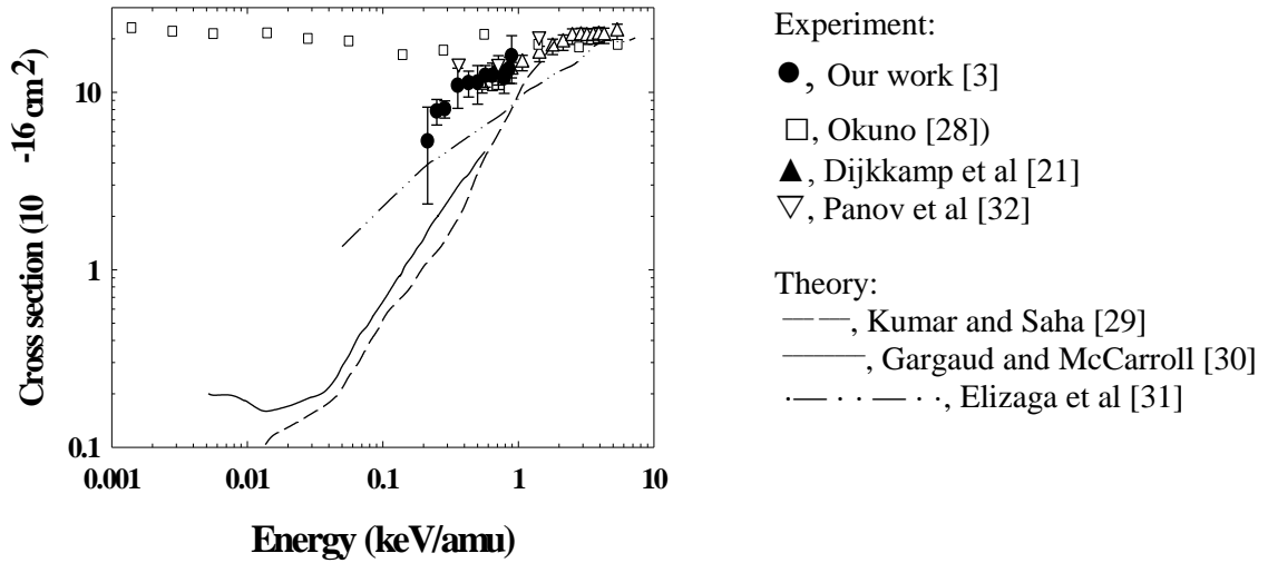
FIG. 11. Total one-electron capture cross-sections for N^{5+} ions in H_2 (from [3]).
