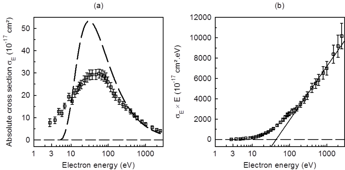
FIG. 7. (a) Total excitation cross-sections ( \sigma_E ) for electron impact upon \text{CD}_4^+ versus electron energy: ( \square ) present measurements and ( - - ) semi-empirical model [5]. (b) Bethe-plot of the excitation cross-section ( \sigma_E ). The full line results from a linear fit using the Bethe-Born formula.
