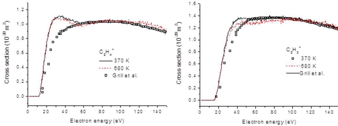
FIG. 23. Absolute partial ionization cross-sections for formation of C_2H_4^+/C_3H_8 and C_2H_3^+/C_3H_8 measured at the gas temperatures of 370 K and 680 K.
