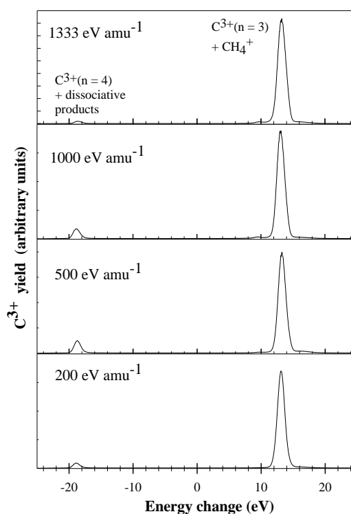
FIG. 24. Energy change spectra for one-electron capture by C^{4+} ions in CH_4 (from [7]).
