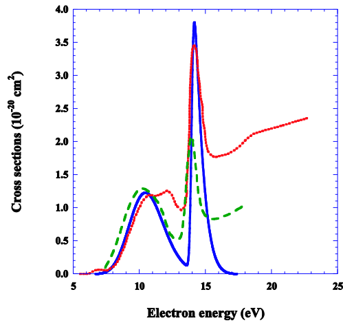
FIG. 10. Comparison between calculated (full curve) and measured cross-sections from refs. [13] (dotted curve) and [14] (dashed
