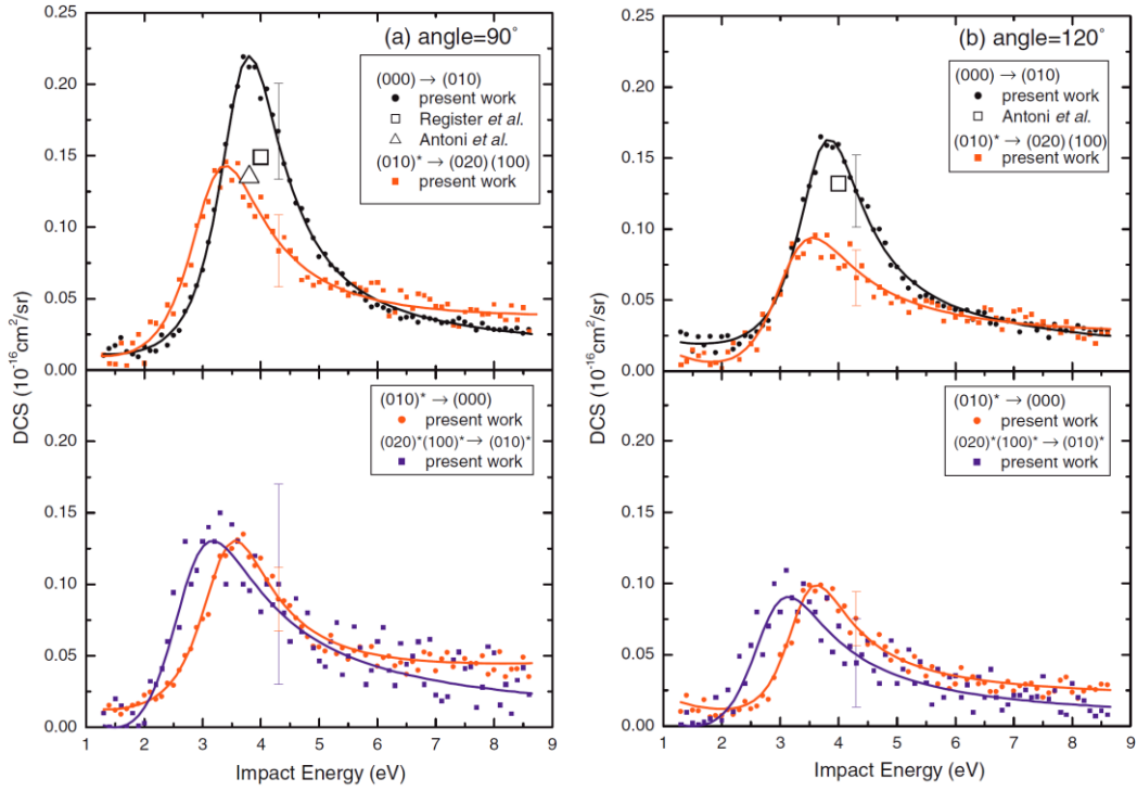
FIG. 9. Vibrational excitation functions for the inelastic (000) \rightarrow (010) and (010)^* \rightarrow (020)(100) transitions and (010)^* \rightarrow (000) and (020)^*(100)^* \rightarrow (010)^* superelastic transitions of \text{CO}_2 at impact energies of 1–9 eV and at scattering angles of (a) 90^\circ and (b) 120^\circ . For detailed information, reference should be made to Ref. [42].
