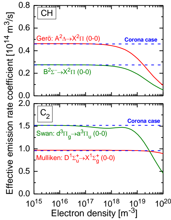
FIG. 10. Effective emission rate coefficients calculated with the CR model in comparison with the corona case for two transitions of the CH and the C_2 molecule at a fixed temperature of T_e = 5 eV.
