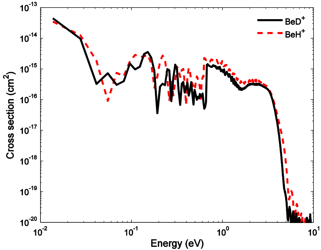
FIG. 7. Total cross-section for dissociative recombination of \text{BeH}^+ and \text{BeD}^+ in their lowest vibrational levels ( \nu = 0 ). (Reproduced from Roos et al. 2009)
