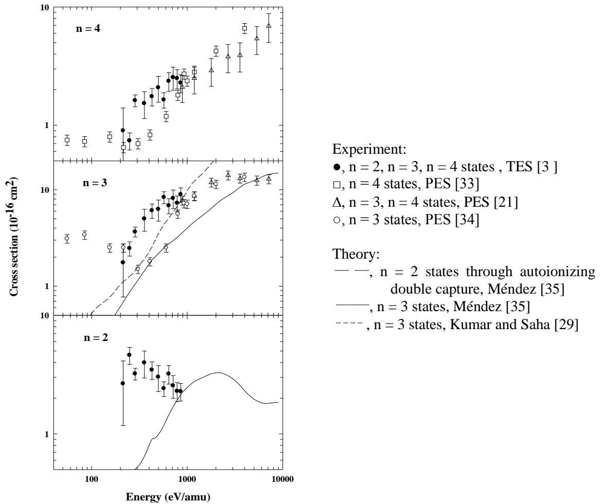
FIG. 12. Cross-sections for selective one-electron capture into n = 2, 3 and 4 states of N^{4+} by N^{5+} ions in H_2 (from [3]).
