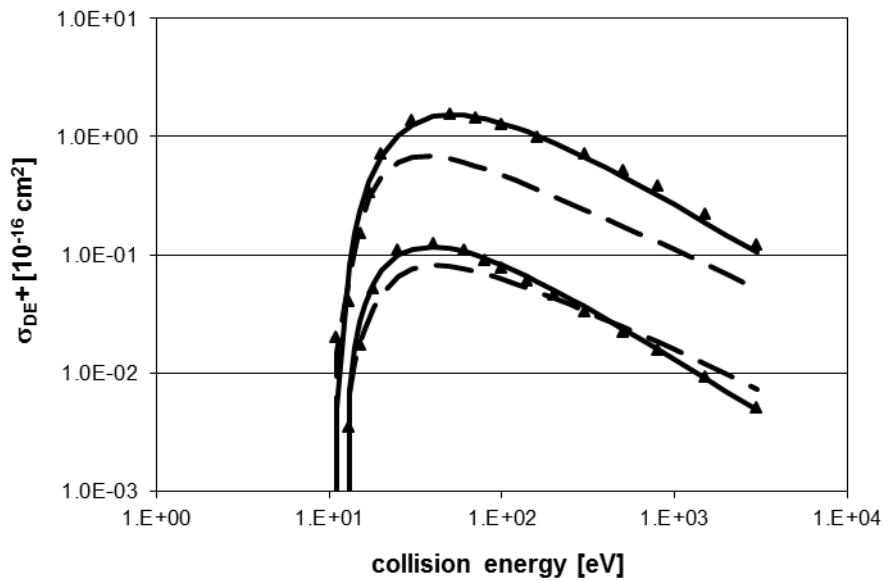
FIG. 6. Dissociative excitation cross-section (in units of 10^{-16} \text{ cm}^2 ) of CH_3^+ ions by electron impact, vs. electron energy (eV). Total H^+ (upper curves) and H_2^+ (lower curves) production channels Triangles: ORNL data. Solid lines: fit to expression (28), ORNL, see text. Dashed lines: fit to LLN data, see Table 7.
