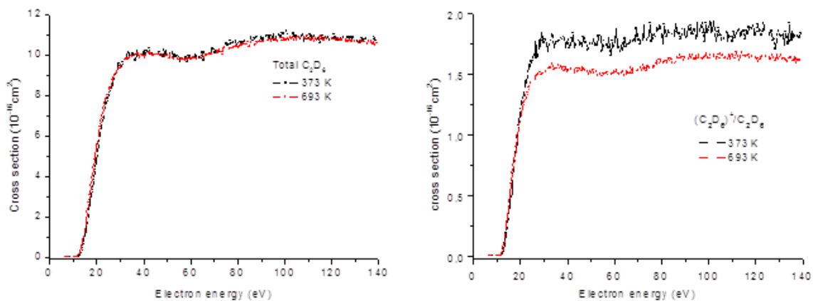
FIG. 11. Absolute total ionization cross-sections formed upon electron impact ionization of C_2D_6 and partial ionization cross-sections for formation of C_2D_6^+/C_2D_6 measured at the gas temperature of 373 K and 693K without the contribution of D^+ and D_2^+ ions.
