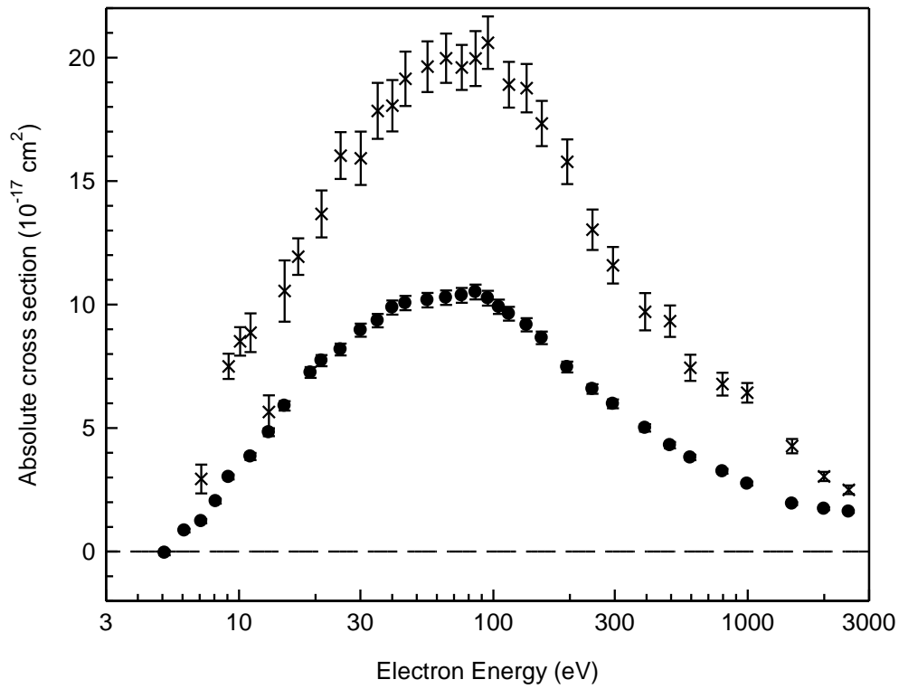
FIG. 1. Absolute cross-sections for the production of D^+ ( \bullet , \sigma_{11} ) and C^+ ( \times , \sigma_{13} ) versus electron energy.
