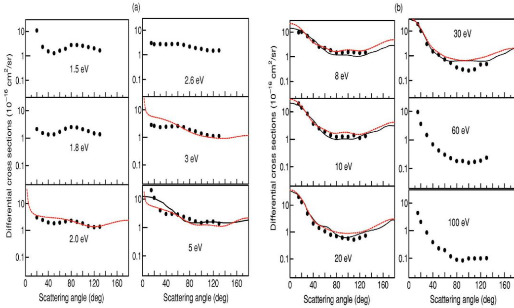
FIG. 3. Electron-impact C_3H_6 experimental (circles) and theoretical (lines) elastic DCSs as functions of the scattering angles in the energy range of (a) 1.5 – 5 eV and (b) 8 – 100 eV. Also included in some panels are the only available DCS results of Winstead et al. (black solid lines). References are in the original paper [34].
