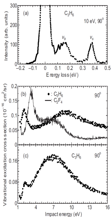
FIG. 6. C 3 H 6 electron impact. (a) Energy loss spectrum at 10 eV and a scattering angle of 90°, and vibrational excitation cross-sections for the (b) bending \nu_b mode, and (c) C-C stretching \nu_s mode.
