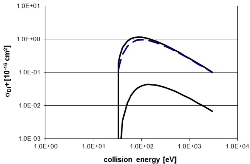
FIG. 7. same as Figure 6, but for dissociative ionization of CH_3^+ ions. Solid lines: fit to expression (28). Total H^+ and H_2^+ production rates derived from Table 11. Dashed line: [30]. Only LLN data are available.
