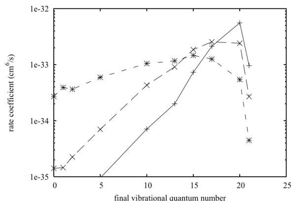
FIG. 5. Deuterium recombination rate coefficients as a function of final vibrational quantum number. at T=300 K (+), T=1\ 000 K (x), T=5\ 000 K (*).
