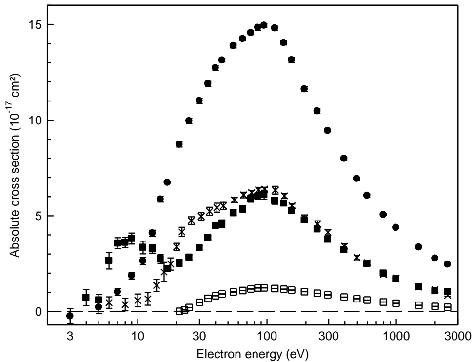
FIG. 2. Absolute cross-sections versus the electron energy for electron-impact on CD_2^+ , for the production of: D^+ ( \sigma_{21} \bullet ), C^+ ( \sigma_{23} \times ) CD^+ ( \sigma_{24} \blacksquare ), and CD_2^+ ( \sigma_{21} \square ).
