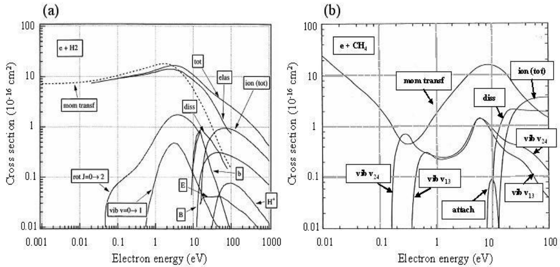
FIG. 1. Electron impact collision cross-sections for (a) H_2 and (b) CH_4 molecules.
