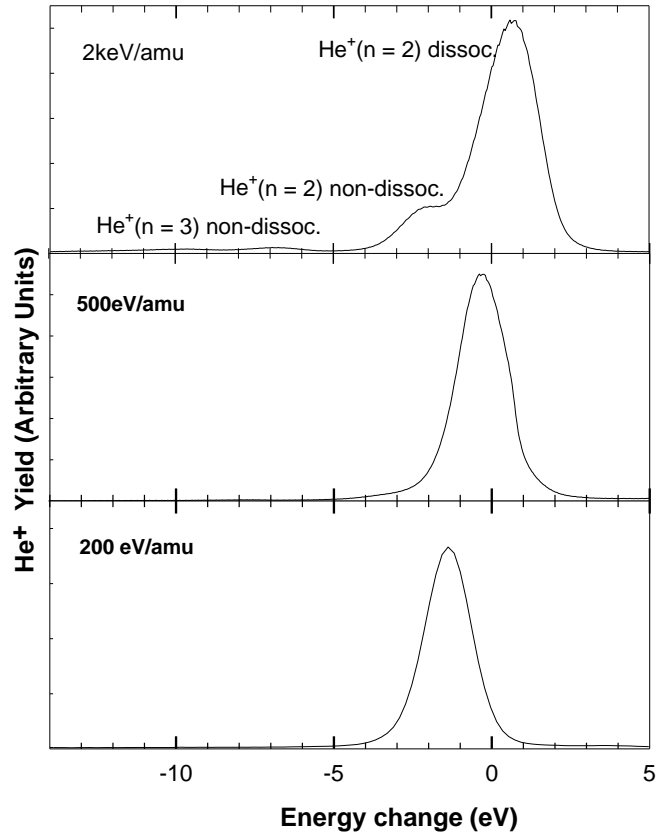
FIG. 19. Energy change spectra for one-electron capture by \text{He}^{2+} ions in \text{C}_2\text{H}_6 (from [5]).
