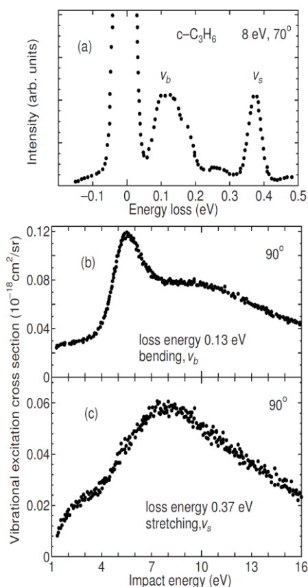
FIG. 5. c -C 3 H 6 electron impact. (a) Energy loss spectrum at 8 eV and a scattering angle of 70°, and vibrational excitation cross-sections for the (b) bending \nu_b mode, and (c) C-C stretching \nu_s mode.
