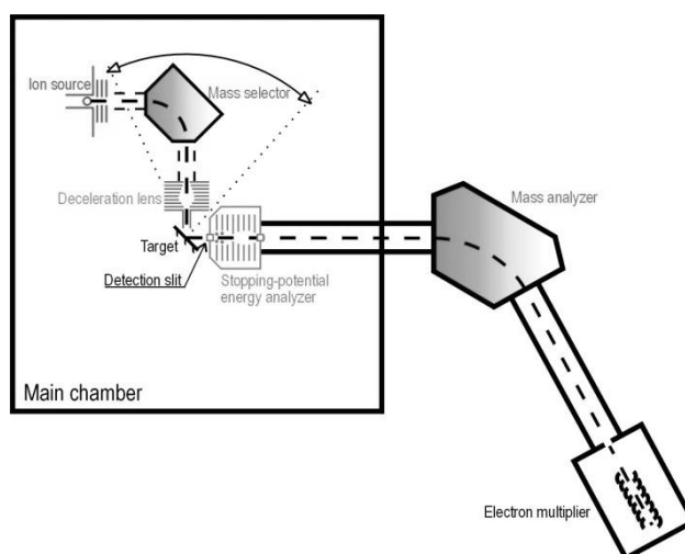
FIG. 1. Schematics of the apparatus EVA.
