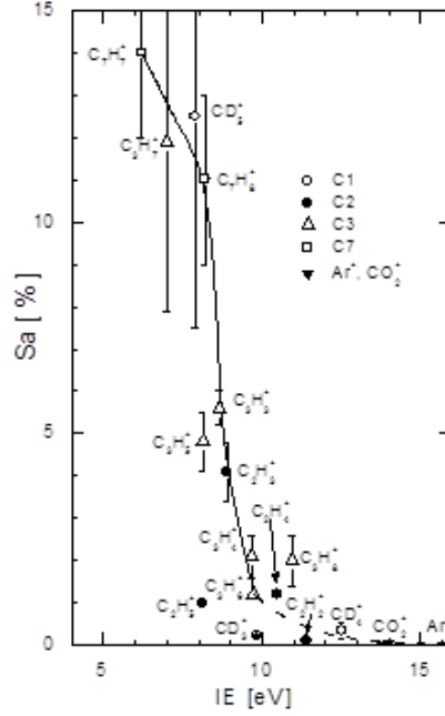
FIG. 3. Dependence S_a - IE for a room-temperature carbon (HOPG) surface.
