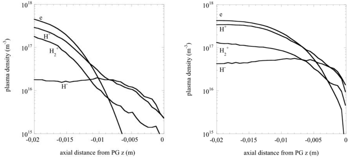
FIG. 14. Axial profiles of the plasma density for the two different line considered: (left panel) extraction hole (line A) and (right panel) PG surface (line B). ( B_{peak}=4 mT and \phi_{PG}=0 V).
