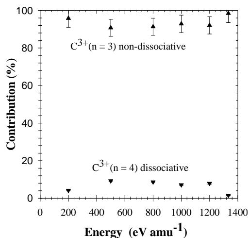
FIG. 25. Measured relative cross-sections for the main product states of \text{C}^{3+} formed in one-electron capture by \text{C}^{4+} ions in \text{CH}_4 (from [7]).
