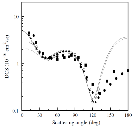
FIG. 4. DCS for elastic e^- - CH_4 scattering at 5 eV. Full line, theoretical data; dot-dashed line, theoretical results of Bettiga et al; full circles, present experimental data; full squares, experimental data of Shyn and Cravens; open circles, experimental data of Boesten and Tanaka; full triangles, experimental data of Bundschu. References are in the original paper [35].
