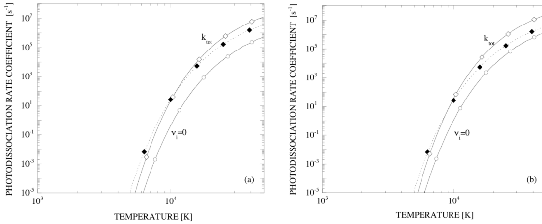
FIG. 7. Photodissociation rate coefficients for H_2(v) in Lyman (a) and Werner (b) systems. The contribution from all vibrational levels (open diamonds) and neglecting vibrational excitation (open circles) have been reported, compared with the rate coefficient in Ref. [22] (close diamonds).
