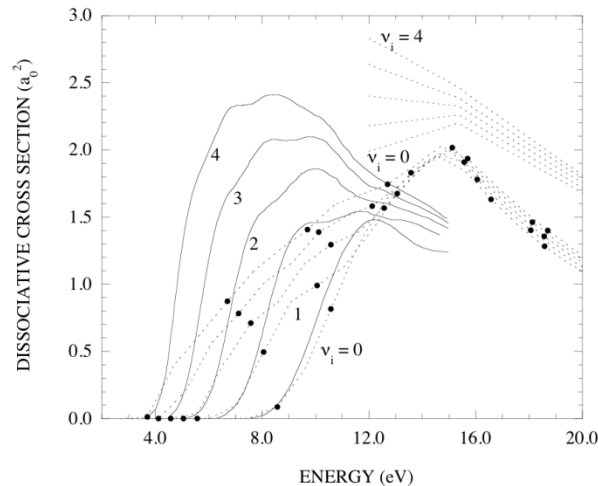
FIG. 1. Cross-section for H_2 direct dissociation through b^3\Sigma_u^+ state, as a function of impact energy, for different initial vibrational levels by different authors. (solid line)-Ref. [6] (dotted line)- Ref. [7] (close circle)-Ref. [8].
