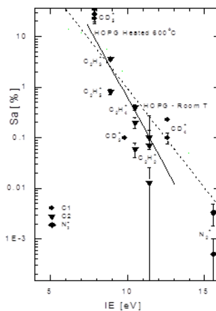
FIG. 5. Dependence S_a - IE in semi-log coordinates for a heated carbon (HOPG) surface.
