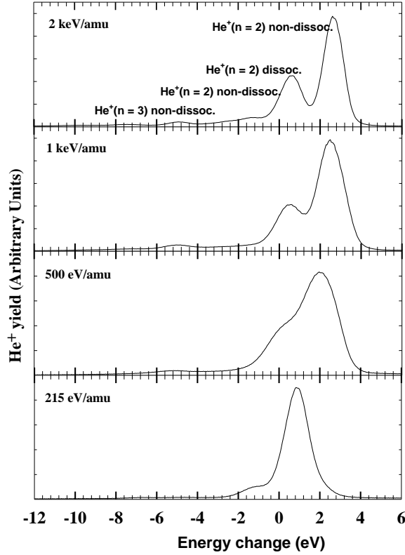
FIG. 18. Energy change spectra for one-electron capture by \text{He}^{2+} ions in \text{C}_2\text{H}_4 (from [5]).
