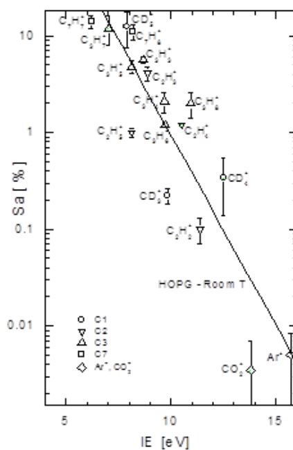
FIG. 4. Dependence S_a - IE in semi-log coordinates for a room-temperature carbon (HOPG) surface.
