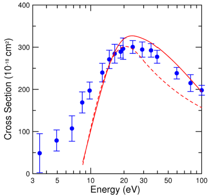
FIG. 3. Absolute cross-sections for the sum of electron-impact dissociative excitation and dissociative ionization of CH^+ ions as a function of center-of-mass energy. The filled circles represent the sum the present measurements for DE+DI producing C^+ fragment ions and the measurements of Ref. [32] for DE producing H^+ fragment ions, both with total absolute uncertainties at a 90% confidence level. The solid and dashed curves represent the predictions of the present molecular dynamics model for DE+DI and DE , respectively.
