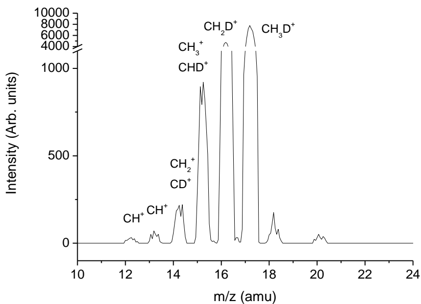
FIG. 6. Mass spectrum of \text{CH}_3\text{D} measured at the gas temperature of 26^\circ\text{C} and the electron energy of 70\text{ eV} .
