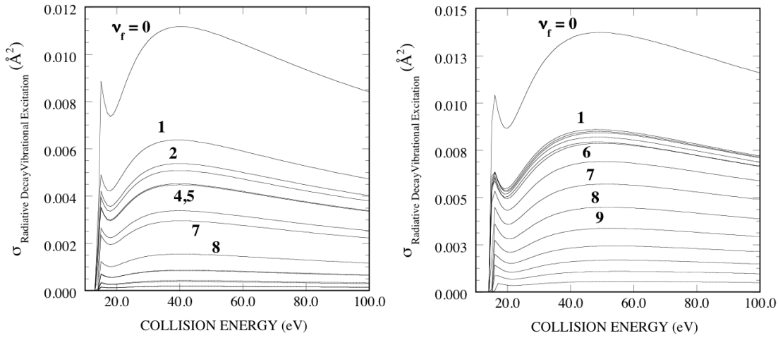
FIG. 2. Cross-section for the process \text{H}_2(\text{X}^1\Sigma_g^+, v_i) + e \rightarrow \text{H}_2^* + e \rightarrow \text{H}_2(\text{X}^1\Sigma_g^+, v_f) + e + h\nu for v_i=0 , as a function of energy, for different v_f : (left panel) \text{H}_2^* = \text{B}'^1\Sigma_u^+ (right panel) \text{H}_2^* = \text{D}^1\Pi_u .
