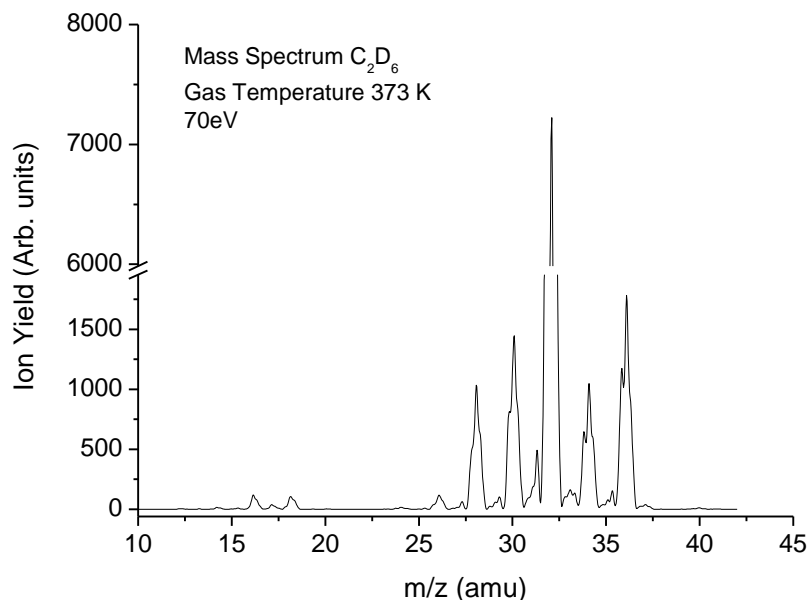
FIG. 10. shows the mass spectrum of C 2 D 6 measured at electron energy of 70 eV and a gas temperature of 373 K.
