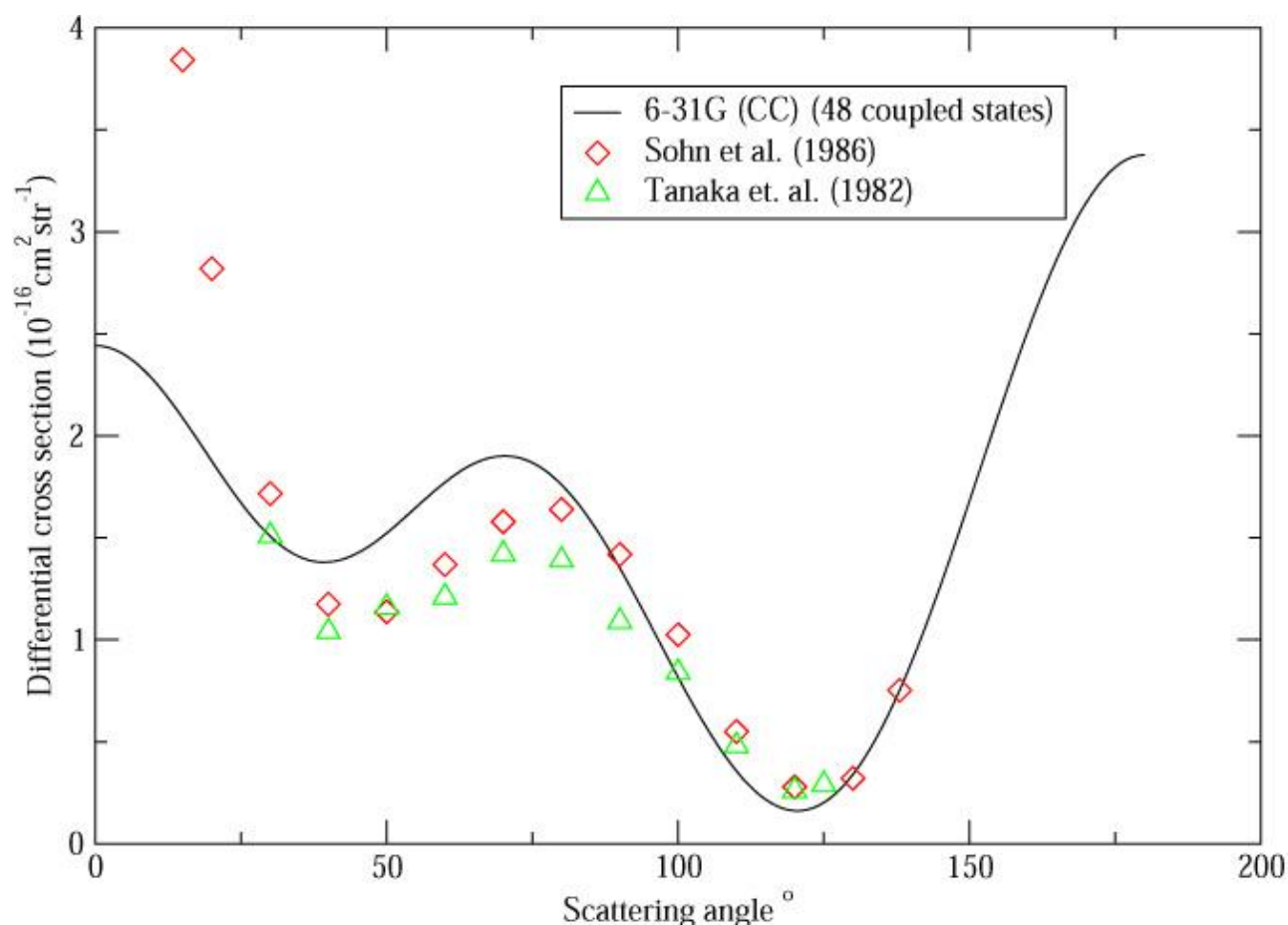
FIG. 2. Differential cross-sections for electron collisions with methane at 5 eV: results of an R-matrix study with 48 coupled states [22] is compared the measurements of Tanaka et al [23] and Sohn et al [24].
