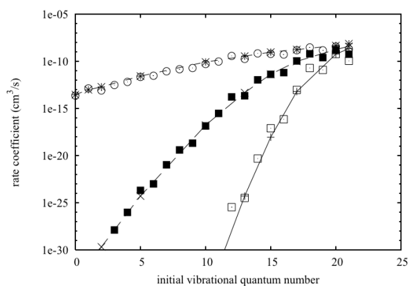
FIG. 4. Deuterium dissociation rate coefficients as a function of initial vibrational quantum number at T=300\text{ K} (+), T=1\,000\text{ K} (x), T=5\,000\text{ K} (*). Markers not connected by lines are results of hydrogen scaled results.
