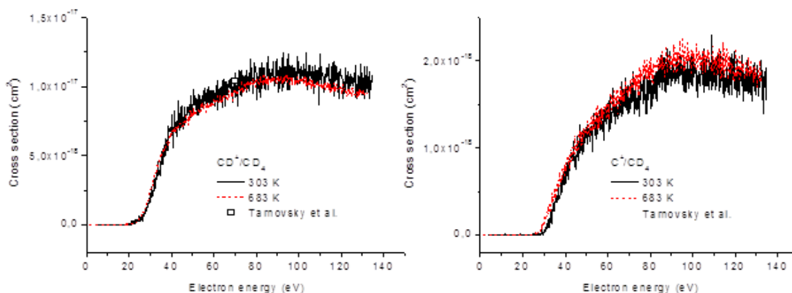
FIG. 5. Partial ionization cross-sections for electron impact ionization of CD^+/CD_4 and C^+/CD_4 measured at the gas temperature of 303 K and 683 K.
