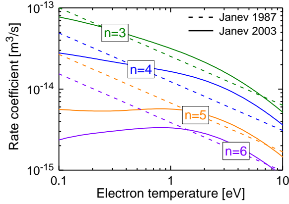
FIG. 6. Comparison of two data sets for the rate coefficient for dissociative recombination of the molecular ion H_2^+ . The quantum numbers refer to the final state of atomic hydrogen.
