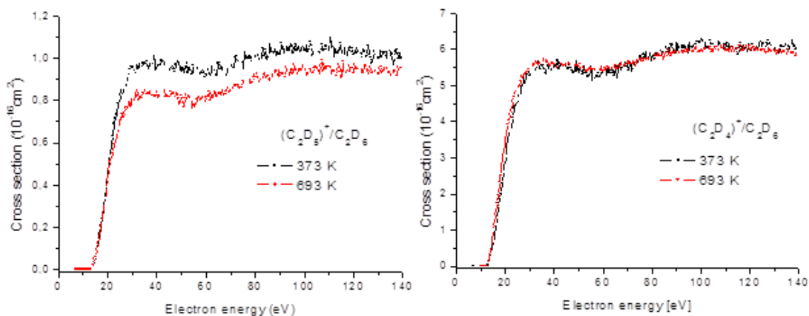
FIG. 17. Absolute partial ionization cross-sections for formation of C_2D_5^+/C_2D_6 and C_2D_4^+/C_2D_6 measured at the gas temperature of 373 K and 693K.
