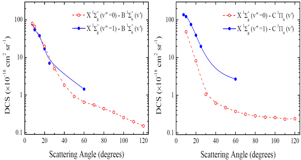
FIG. 10. DCS for excitation of the B^1\Sigma_u + (v') and C^1\Pi_u(v') states from the X^1\Sigma_g + (0) and X^1\Sigma_g + (1) ground state levels of H_2 at an impact energy of 40 eV. For detailed information, reference should be made to Ref. [43].
