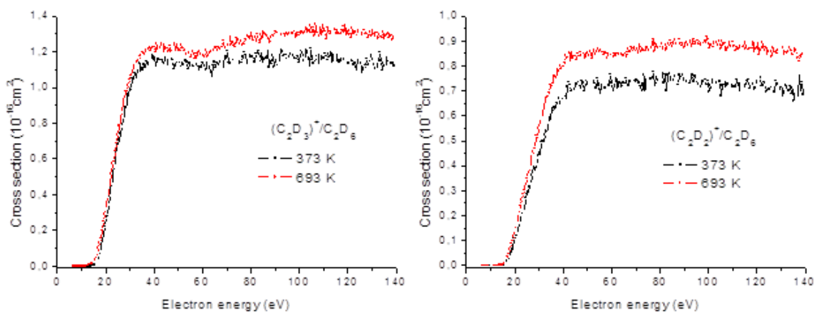
FIG. 18. Absolute partial ionization cross-sections for formation of C_2D_3^+/C_2D_6 and C_2D_2^+/C_2D_6 measured at the gas temperature of 373 K and 693K.
