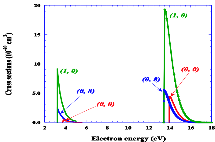
FIG. 11. Comparison between DEA cross-sections occurring through the ^2\Sigma_u^+ ground state (left) and the ^2\Sigma_g^+ Rydberg state (right) of the H_2^- ion. (see text).
