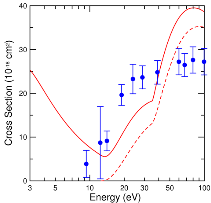
FIG. 8. Absolute cross-sections for the production of \text{C}^+ fragment ions by electron-impact dissociation of \text{CH}_3^+ ions as a function of center-of-mass energy. The filled circles are the present measurements with total absolute uncertainties at a 90% confidence level, while the dashed curve represents the predictions of Ref. [21] and the solid curve represents the data found in the HYDKIN database [46].
