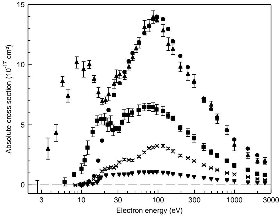
FIG. 3. Absolute cross-sections versus the electron energy for electron-impact on CD_3^+/(CH_3^+) for the production of: D^+ ( \sigma_{31} ●), H_2^+ ( \sigma_{32} ▼), C^+ ( \sigma_{33} ×), CH^+ ( \sigma_{34} ■) and CD_2^+ ( \sigma_{35} ▲).
