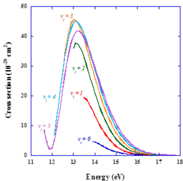
FIG. 12. DEA cross-sections for process (8) where v_i = 0-5 .
