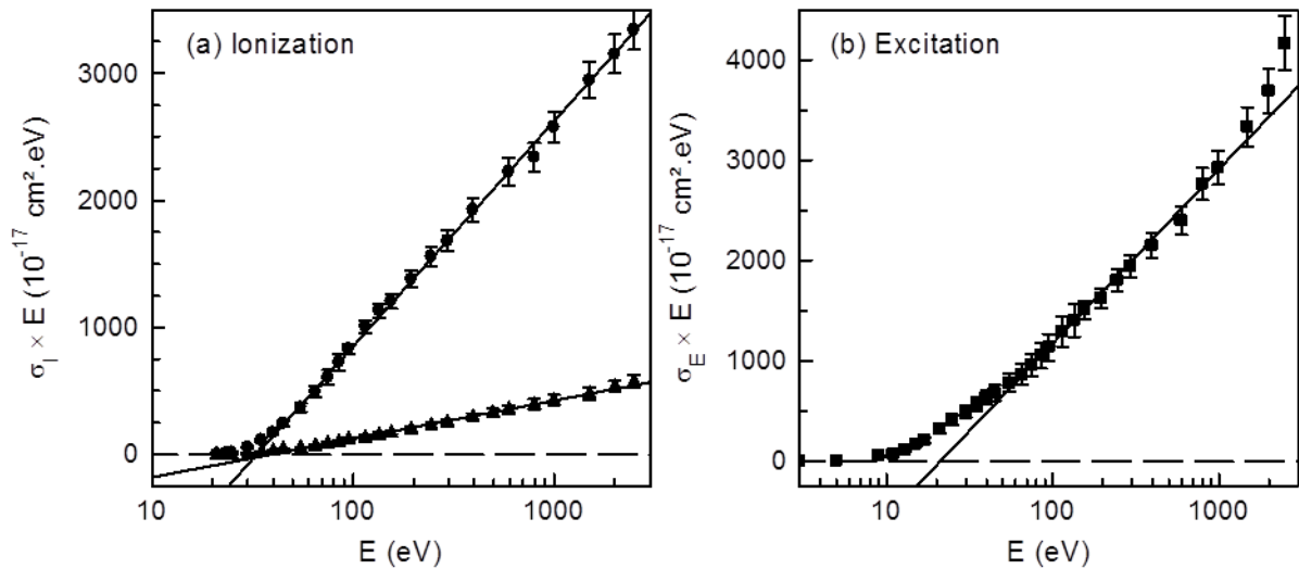
FIG. 8. Bethe-plot of the (a) total ionization cross-section ( \bullet \sigma_I ) together with the single ionization cross-section ( \blacktriangle \sigma_{SI} ), and of the (b) total excitation cross-section ( \blacksquare \sigma_E ) of \text{CD}_2^+ . Each full line results from a linear fit using the Bethe-Born formula.
