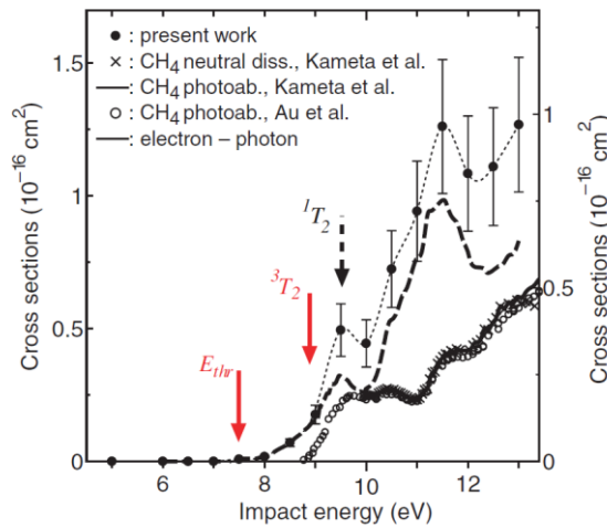
FIG. 7. Absolute cross-sections for \text{CH}_3 radical production. Also included are the photon impact results from literature. The arrows show the threshold energy E_{thr} and the ^3T_2 and ^1T_2 state peaks. The dashed curve is the difference between the current neutral \text{CH}_3 and the photon impact total neutral dissociation cross-sections. For detailed information, reference should be made to Ref. [37].
