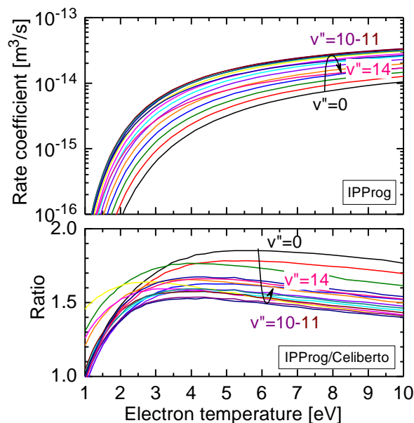
FIG. 4. Excitation rate coefficient for the X \ ^1\Sigma_g^+ to B \ ^1\Sigma_u^+ transition of the hydrogen molecule calculated with IPProg . Ratio of the rate coefficient from IPProg calculations to the rate coefficient calculated by Celiberto [39] using the semi-classical impact parameter method for molecules [33].
