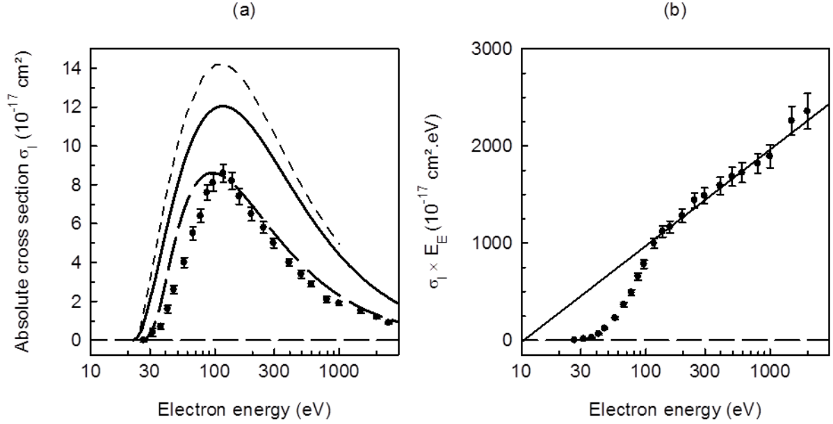
FIG. 6. (a) Total ionization cross-sections ( \sigma_i ) for electron impact upon CD_4^+ versus electron energy: ( \bullet ) present measurements; (—) BEB formalism [6]; (---) DM formalism [15] and (— —) semi-empirical model [5]. (b) Bethe-plot of the ionization cross-section ( \sigma_i ). The full line results from a linear fit using the Bethe-Born formula.
