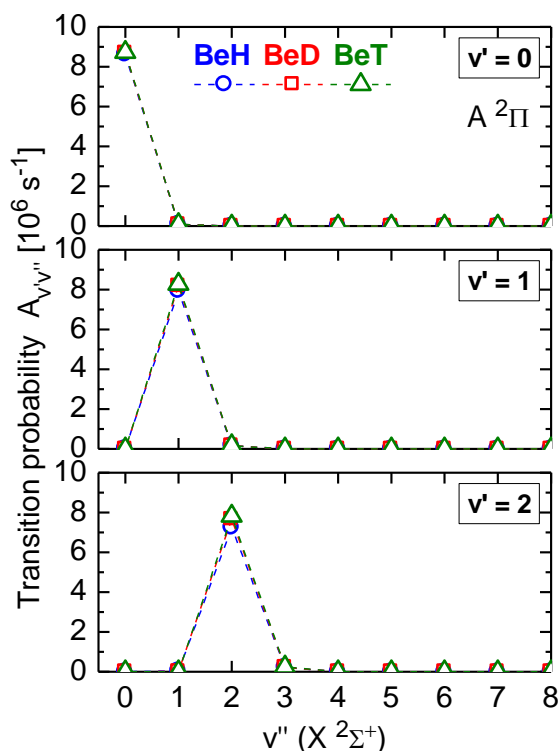
FIG. 3. Vibrationally resolved transition probabilities for the first electronic state into the ground state of BeH, BeD and BeT: A(v'=0, 1, and 2) into X(v''=0-8).
