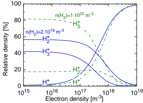
FIG. 7. Calculation of the hydrogen ion composition for two molecular hydrogen densities.
