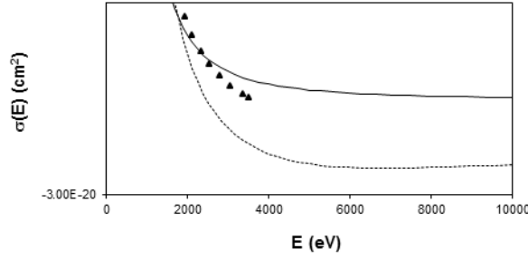
FIG. 3. Example of negative cross-sections at large electron energies in original database, shown here for double ionization of C_3H_8 . Triangles: original data, from [14]. dotted line: original fit, loc.cit., solid line: corrected fit according to procedure described in text.
