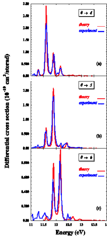
FIG. 7. RVE cross sections for the 0 \rightarrow v_f = 4-6 excitation.
