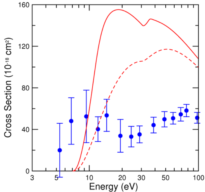
FIG. 6. Absolute cross-sections for the production of CD_2^+ fragment ions by electron-impact dissociation of CD_3^+ ions as a function of center-of-mass energy. The filled circles are the present measurements with total absolute uncertainties at a 90% confidence level, while the dashed curve represents the predictions of Ref. [21] and the solid curve represents the data found in the HYDKIN database [46].
