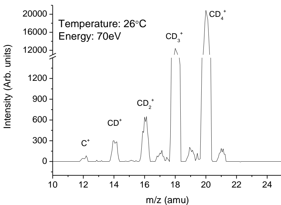
FIG. 2. Mass spectrum of CD_4 measured at the gas temperature of 303K and the electron energy of 70 eV.
